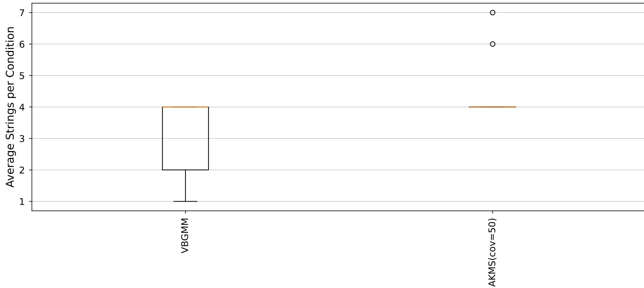
YARA Rules Average Strings per Condition Distribution (Cluster5_Size23 dataset)
